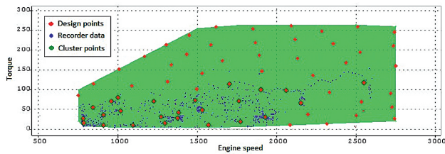
Figure 1: Speed and load area for a global DOE
