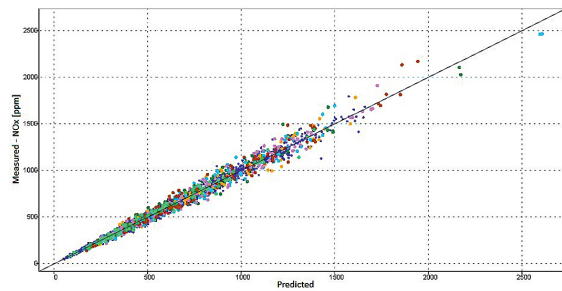
Figure 2: Measured vs. predicted NO x
